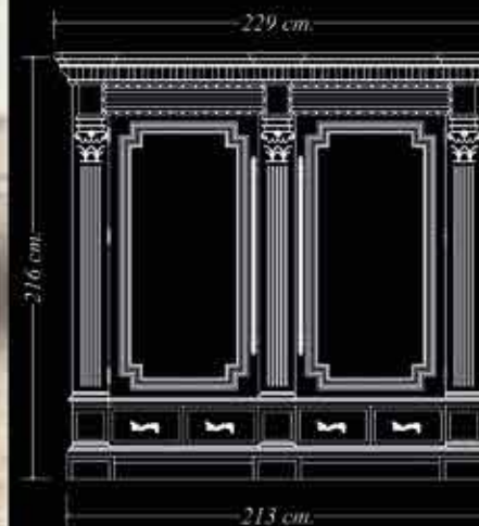
455 Descartes Buffet Front View
